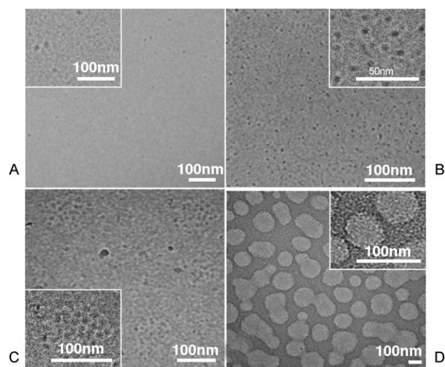
Figure 3. Cryo-TEM micrographs of rec1-resilin for solutions of A) 0.3 \text{ mg mL}^{-1} at 20^\circ\text{C} , B) 0.3 \text{ mg mL}^{-1} just below UCST ( 4^\circ\text{C} ), C) 0.3 \text{ mg mL}^{-1} above LCST, and D) 10 \text{ mg mL}^{-1} at 4^\circ\text{C} .
